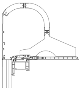
ROLLADEN – REVISION INNEN
