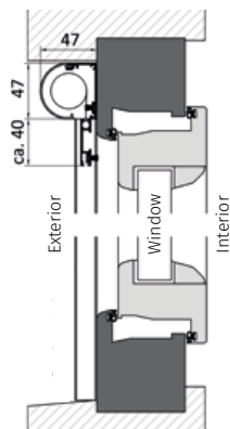
Installation on the window frame (vertical)
